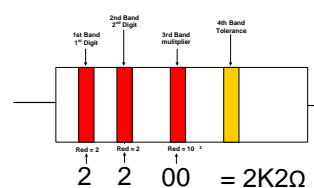
2K2Ω resistor
